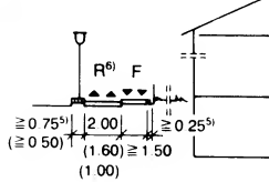
② Cycle path running alongside the road
